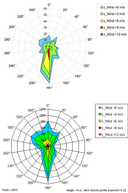
Figure 10: Wind rose
