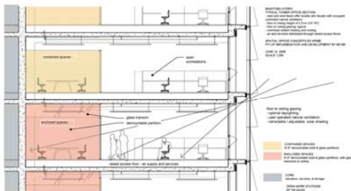
Fig 12 Typical loft sections showing daylight penetration
