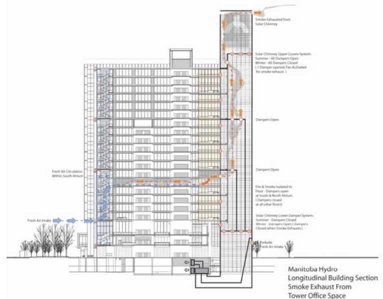
Fig 5: Charette 3: Refinement of Options: shown here the Comfort Tower Option
